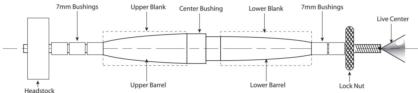
Diagram B / Turning the Wood Blanks
