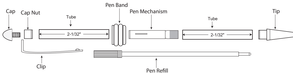
Diagram A / Parts Layout
