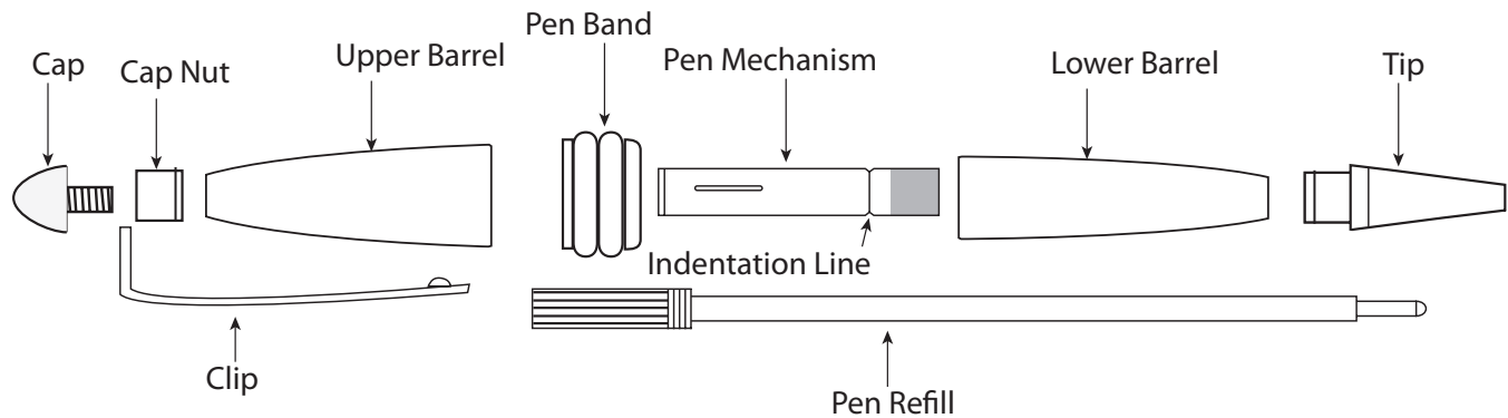
Diagram C / Assembly
