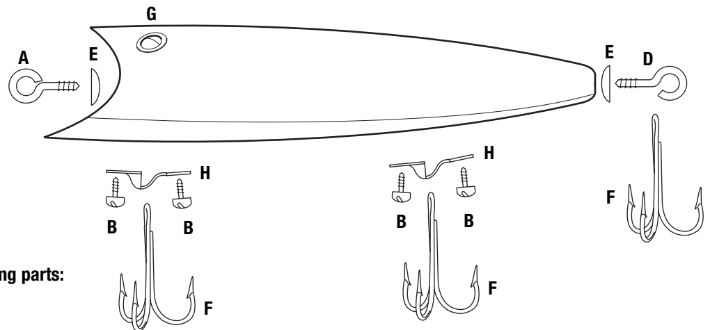
Diagram C - Assembly
