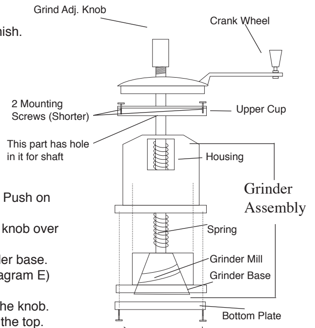
Diagram C Grind Assembly
