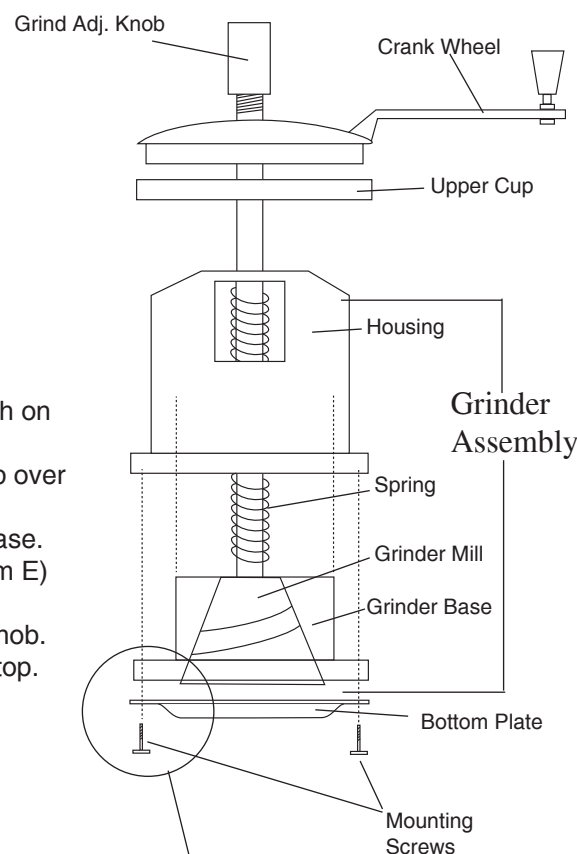
Diagram C Grind Assembly
