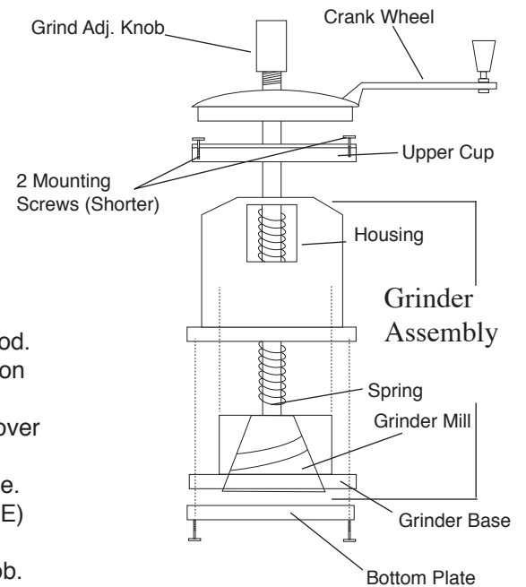
Diagram C Grind Assembly
