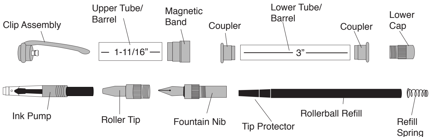
DIAGRAM A / PARTS LAYOUT
