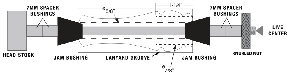
DIAGRAM B / TURNING THE BLANK
