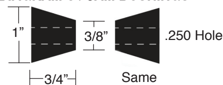
DIAGRAM C / JAM BUSHINGS
