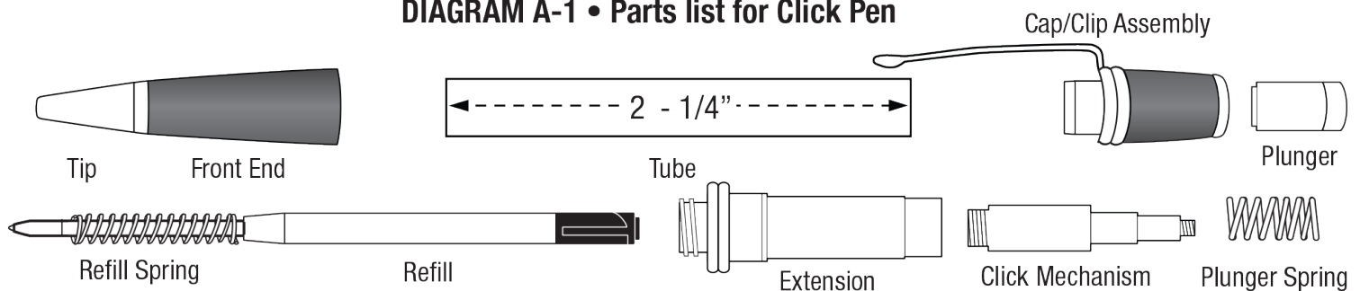
DIAGRAM A-1 • Parts list for Click Pen
