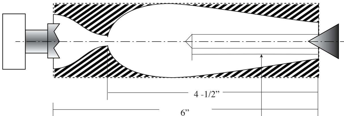
DIAGRAM B / TURNING THE HANDLE BLANK
