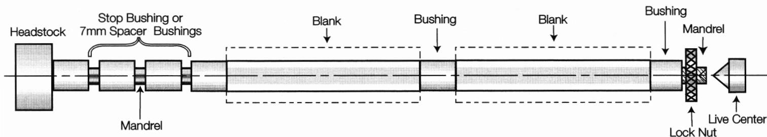
Diagram B / Turning The Blanks (2 Kits at one time)
