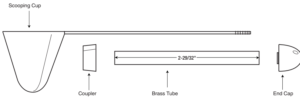
Diagram A- Parts Layout
