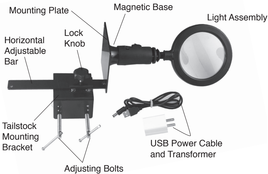
DIAGRAM A / PARTS LAYOUT
