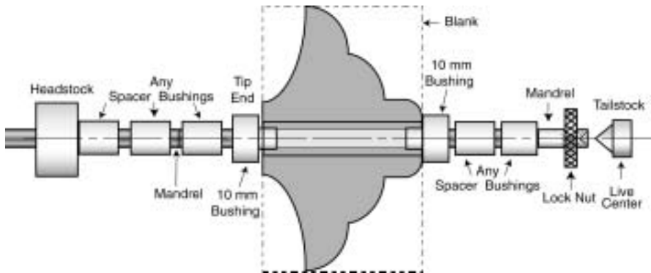
Diagram B - Turning the Blank
