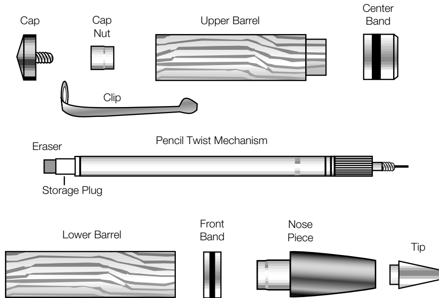
Diagram C - Assembly
