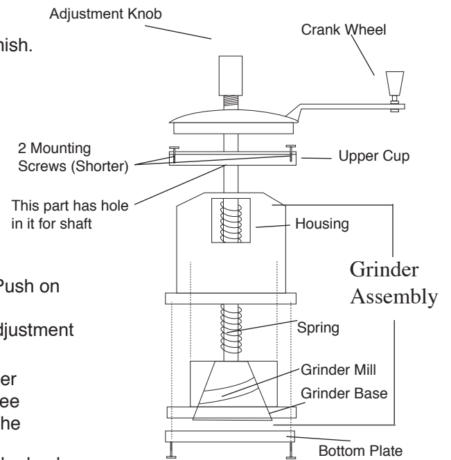
Diagram C Grind Assembly
