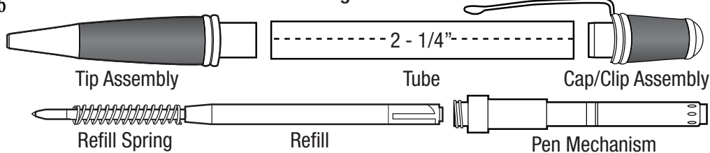
Diagram A - Parts list
