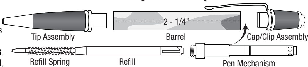
Diagram C - Assembly
